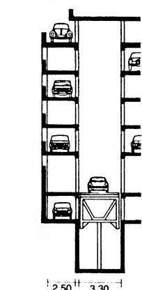
⑫ Transverse stacking
